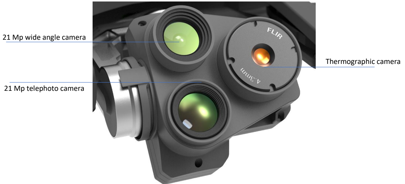
Fig. 11: Triple camera module
