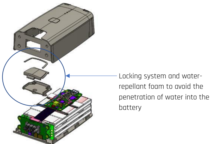
Fig. 17: Waterproof mechanical cover
