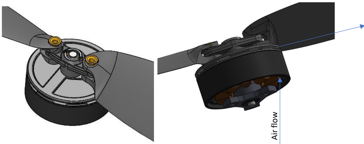
Fig. 4: Motor covers
